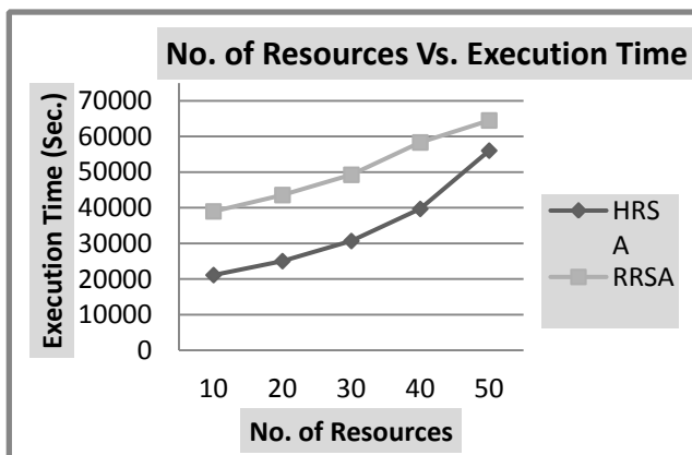
Fig 2: No of Resources Vs. Execution Time
